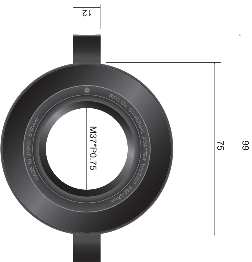
UAC3500 Universal Adapter
