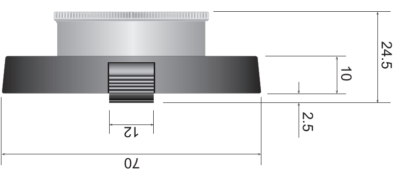
Macro lens + UAC3500 Universal Adapter
