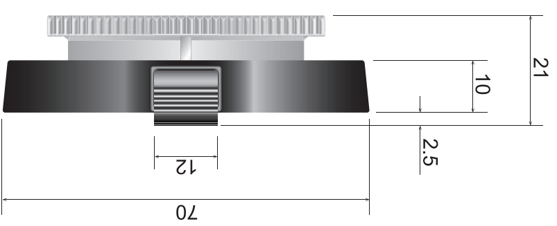
Macro lens + UAC2000 Universal Adapter
