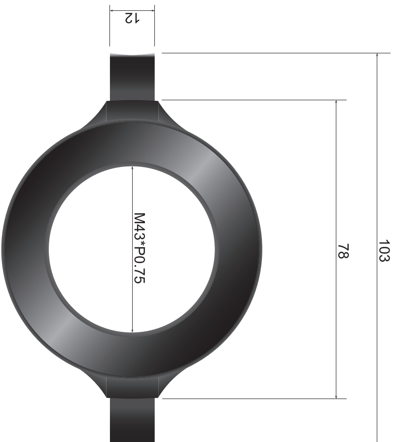
UAC2000 Universal Adapter
