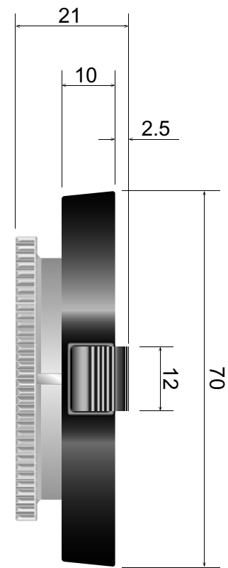
Macro lens + UAC2000 Universal Adapter
