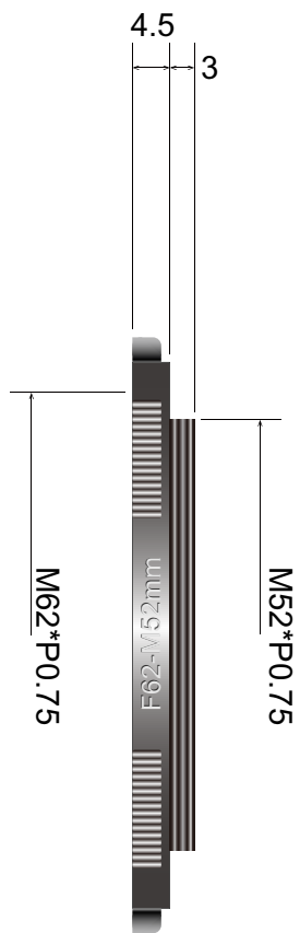
RA6252 Adapter ring
