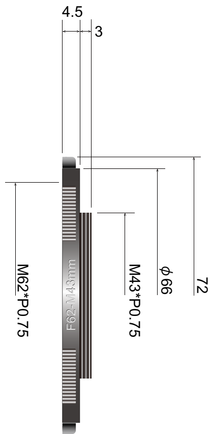
RA6243 Adapter ring
