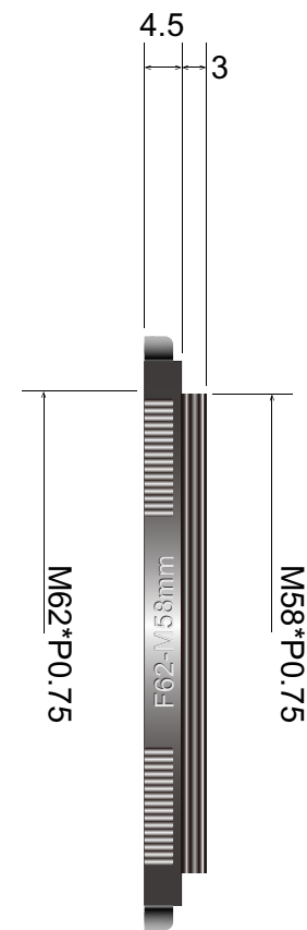
RA6258 Adapter ring
