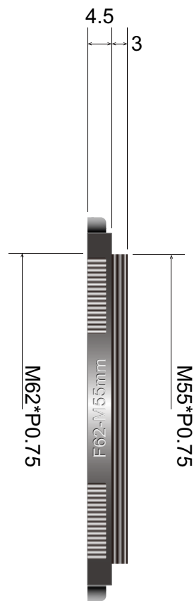
RA6255 Adapter ring
