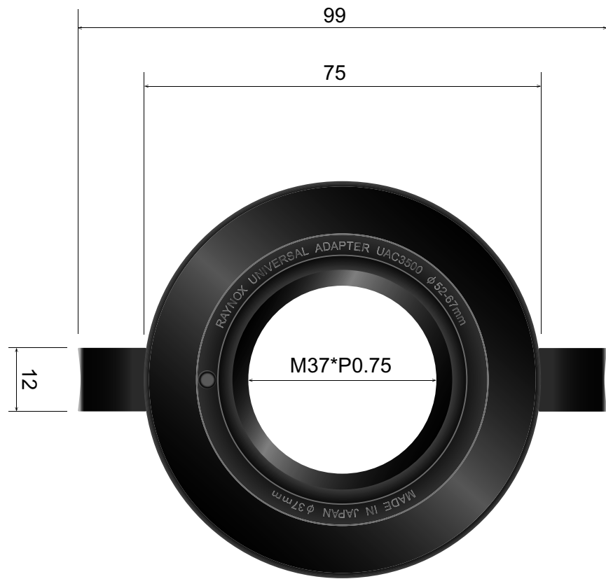
UAC3500 Universal Adapter
