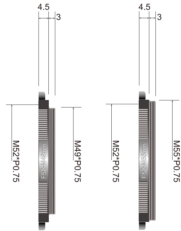
RA5249B Adapter ring
